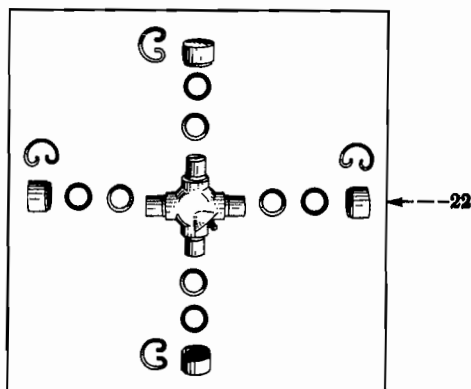
FIG. 06-32 — PROPELLER SHAFT (Spicer 1350 Series) (Transmission To Transfer Case) (R-140-4x4, R-160-4x4)
