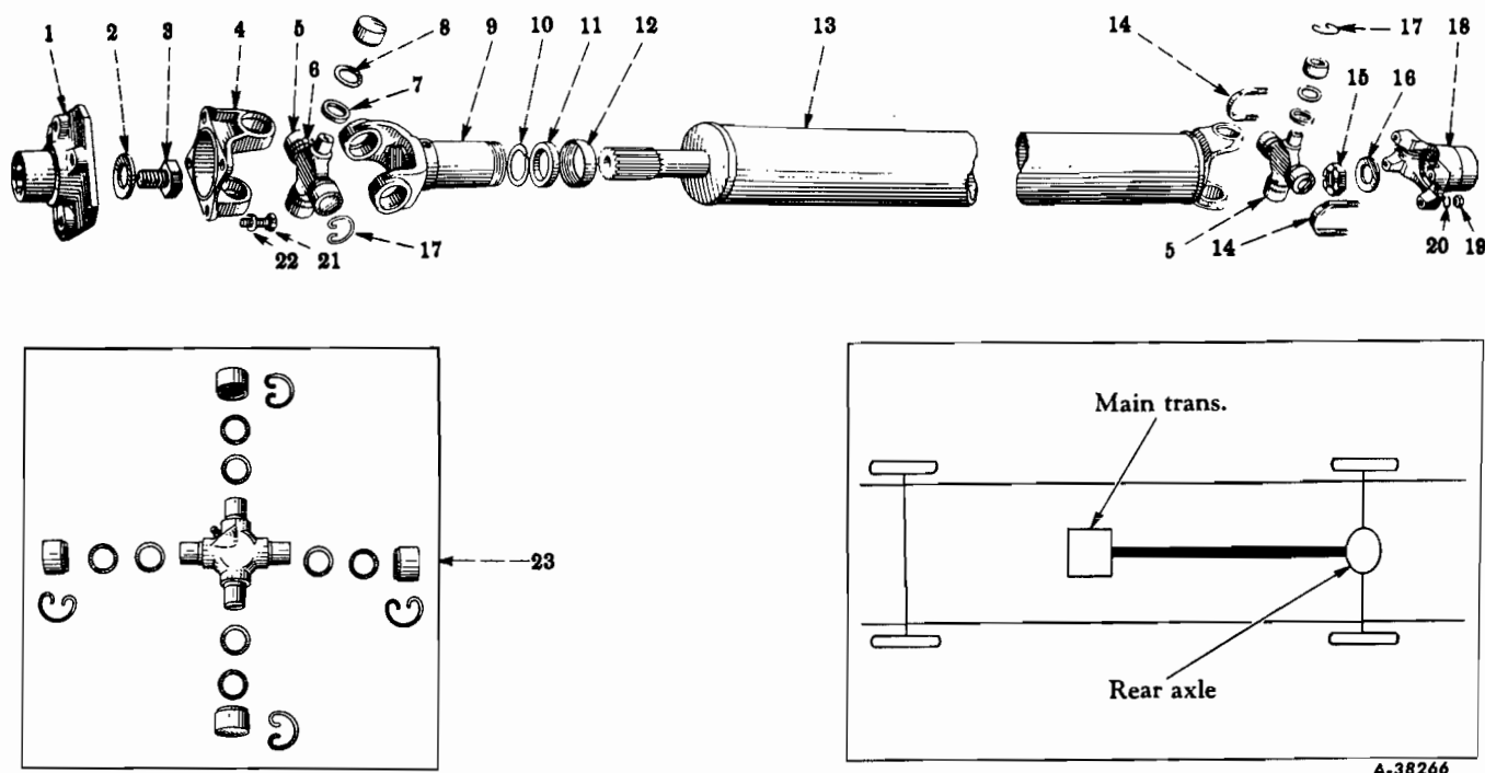
FIG. 06-2 — PROPELLER SHAFT (Spicer 1260 Series) (Transmission To Rear Axle) (R-100 Series - With Transmission Code 1374)
