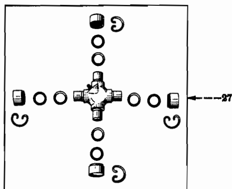
FIG. 06-29 — PROPELLER SHAFT (Spicer 1410, 1350 Series) (Transmission To Rear Axle) (RC-160 Series - With 106" W.B.) (Below 1052 - Spicer 1410 Series) (1052 Up - Spicer 1350 Series)
