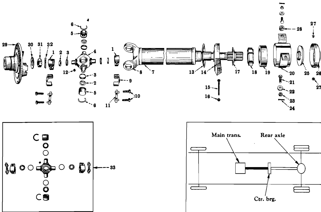
FIG. 06-21 — PROPELLER SHAFT (Mechanics 4-CSR) (Transmission To Center Bearing) (R-150 Series)
