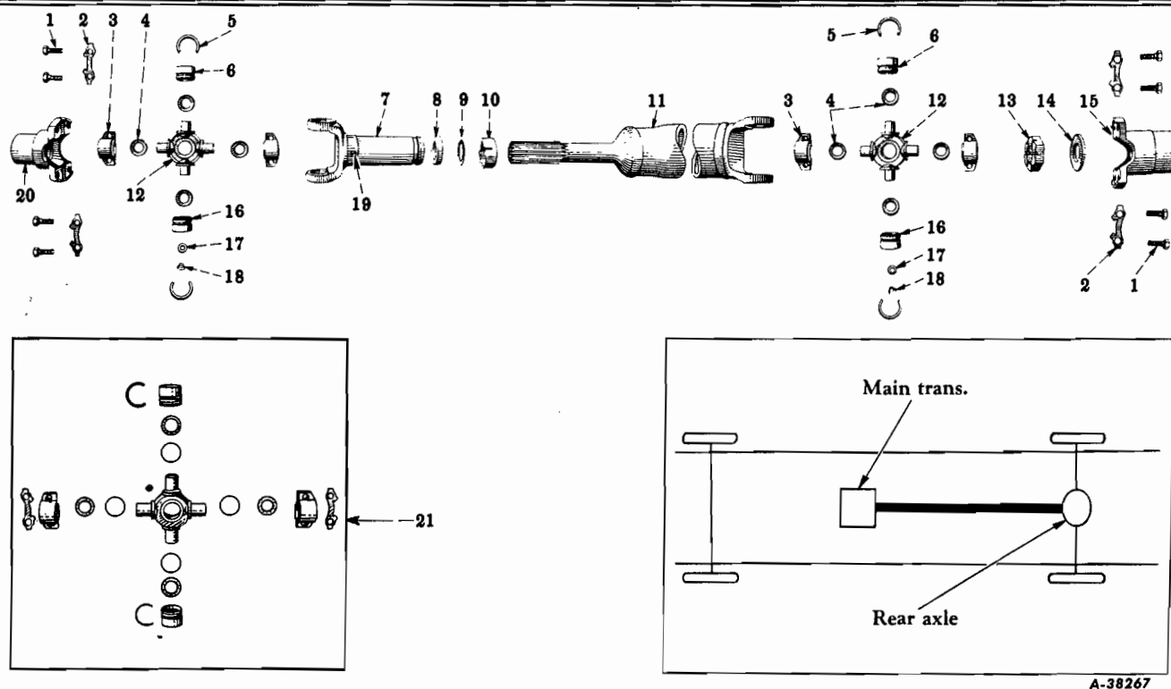
FIG. 06-5 - PROPELLER SHAFT (Mechanics 2-LCR) (Transmission To Rear Axle) (R-110 Series - With Transmission Code 1383)
