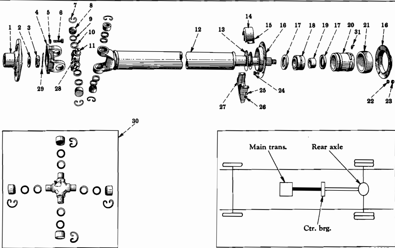
FIG. 06-25 - PROPELLER SHAFT (Spicer 1410, 1350 Series) (Transmission To Center Bearing) (R-160 Series - With 208" W.B.) (9400 Up - Spicer 1350 Series) (Below 9400 - Spicer 1410 Series)
