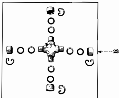
FIG. 06-6 – PROPELLER SHAFT (Spicer 1260, 1270 Series) (Transmission To Rear Axle) (R-110, R-120 Series - For 115" W.B., Spicer 1260 Series, With Transmission Codes 1301, 1302, 1303, 1348) (R-110, R-120 Series - For 127" W.B., Spicer 1270 Series, With Transmission Codes 1301, 1302, 1303, 1348)
