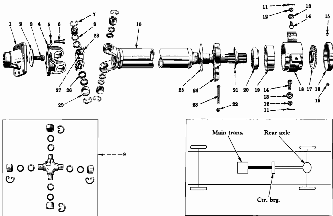
FIG. 06-14 — PROPELLER SHAFT (Spicer 1310 Series) (Transmission To Center Bearing) (R-130 Series - For 134" W.B., With Transmission Codes 1302, 1303, 1320, 1374)
