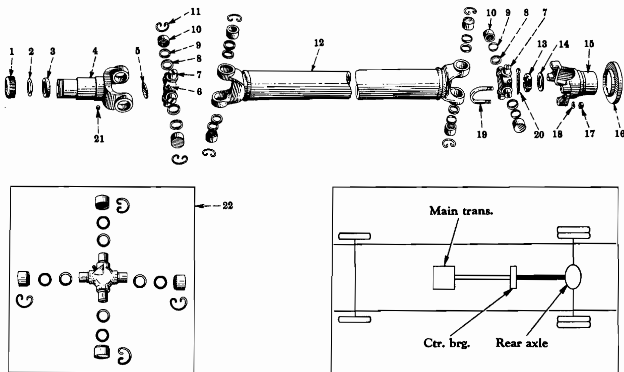
FIG. 06-27 — PROPELLER SHAFT (Spicer 1410, 1350 Series) (Center Bearing To Rear Axle) (R-160 Series - With 130, 142, 154, 172, 190" W.B.) (Below 9400 - Spicer 1410 Series) (9400 Up - Spicer 1350 Series)
