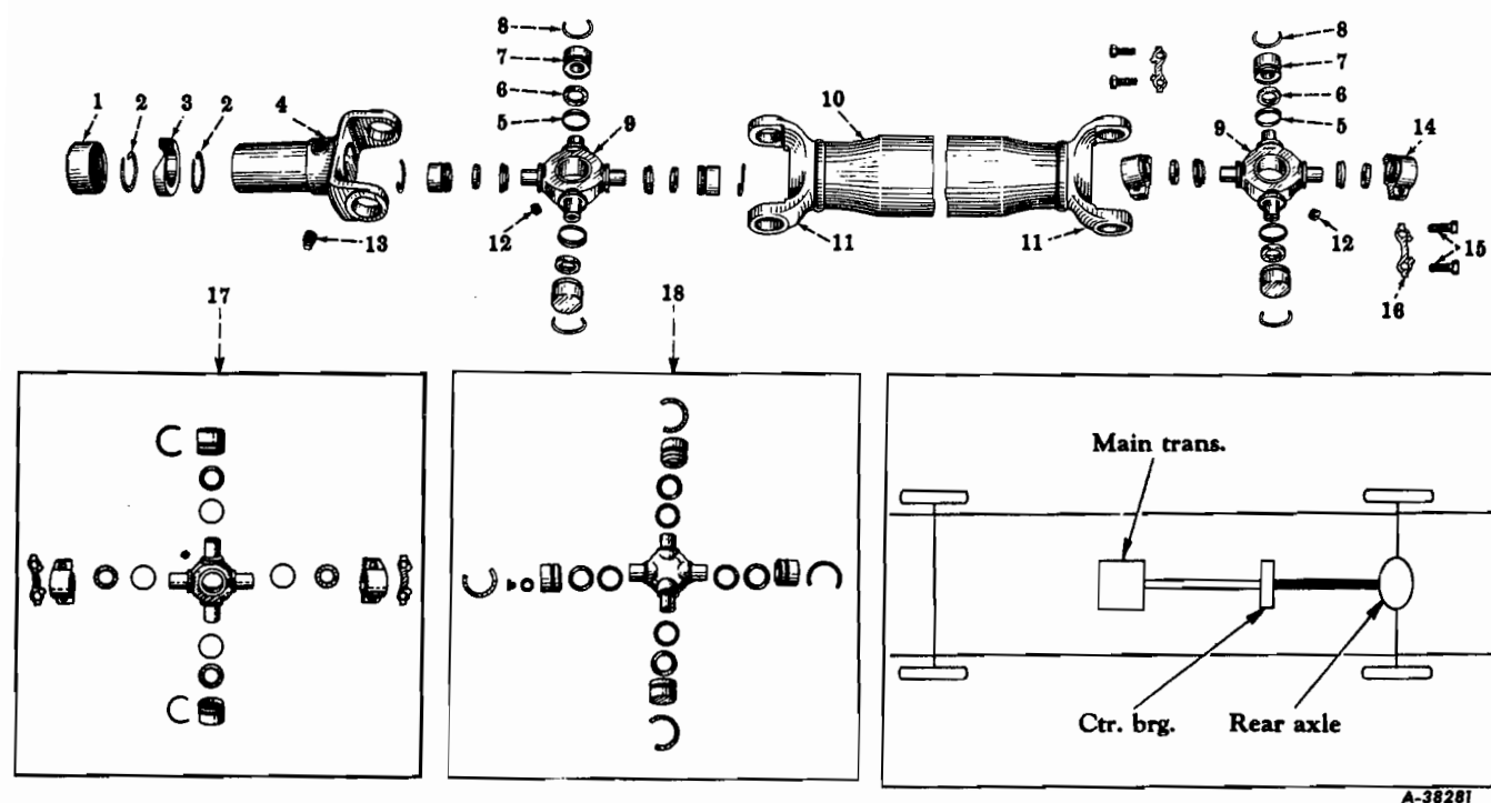
FIG. 06-19 — PROPELLER SHAFT (Mechanics 4-CR) (Center Bearing To Rear Axle) (R-130 Series - For 134" W.B., With Transmission Codes 1302, 1303, 1320)
