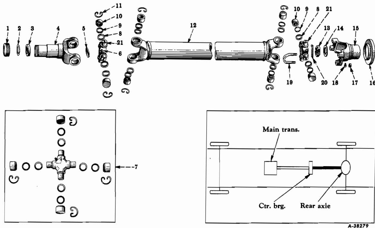
FIG. 06-17 — PROPELLER SHAFT (Spicer 1310 Series) (Center Bearing to Rear Axle) (R-130 Series - For 134" W.B., Transmission Codes 1302, 1303, 1320, 1374)
