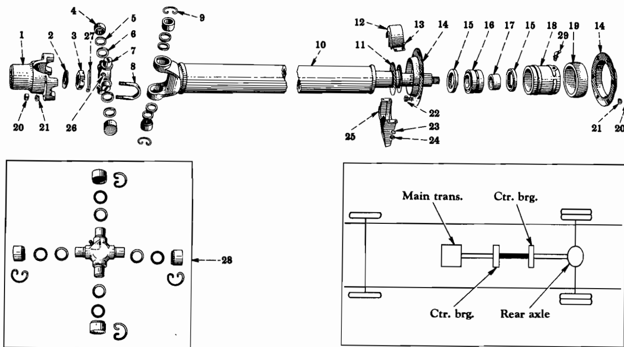
FIG. 06-26 — PROPELLER SHAFT (Spicer 1410, 1350 Series) (Center Bearing To Center Bearing) (R-160 Series - With 208" W.B.) (Below 9400 - Spicer 1410 Series) (9400 Up - Spicer 1350 Series)
