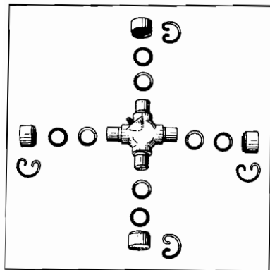
FIG. 06-13 – PROPELLER SHAFT (Spicer 1310 Series) (Transmission To Rear Axle) (R-130 Series – For 122" W.B., With Transmission Codes 1302, 1303, 1320, 1374)
