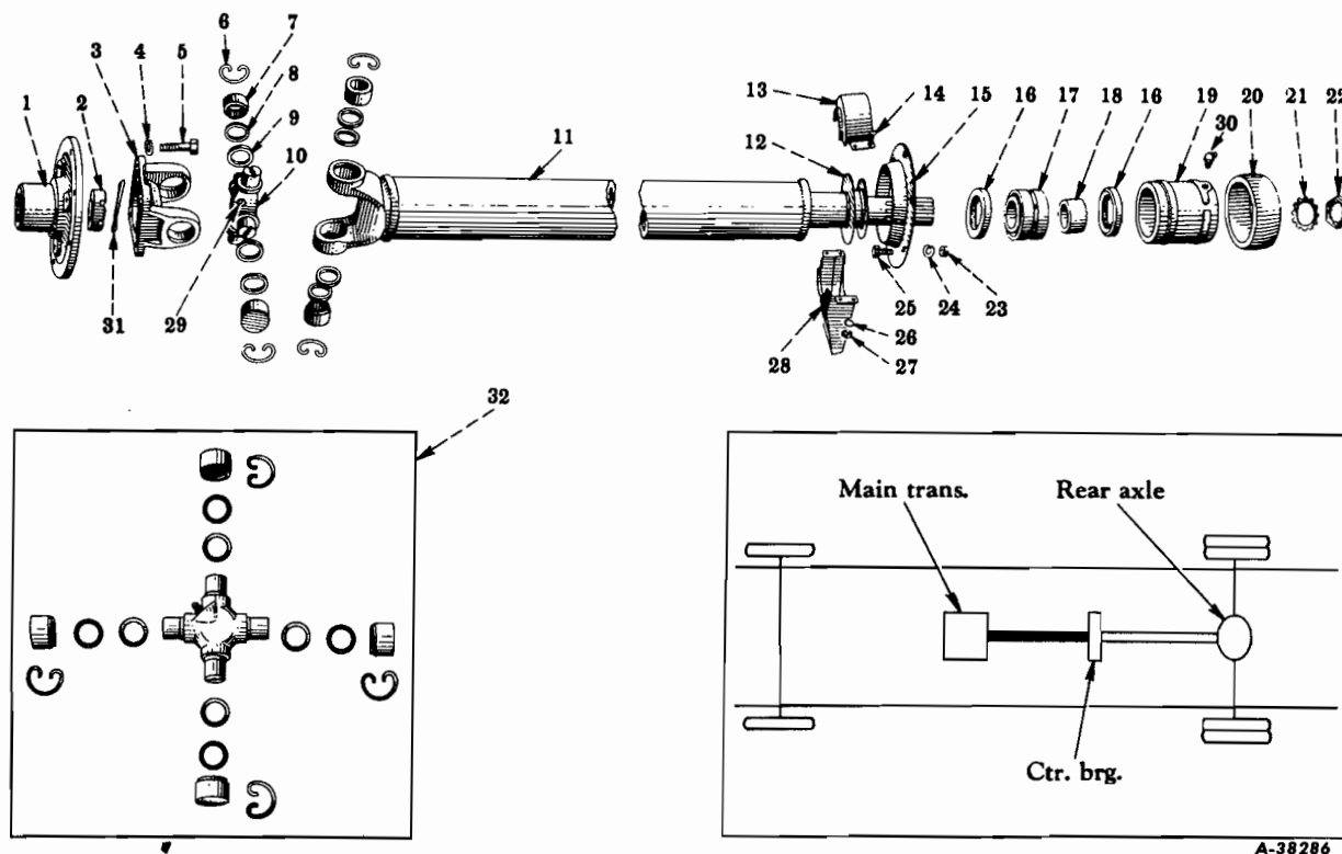
FIG. 06-24 — PROPELLER SHAFT (Spicer 1410, 1350 Series) (Transmission To Center Bearing) (R-160 Series - With 130, 142, 154, 172, 190" W.B.) (Below 9400 - Spicer 1410 Series) (9400 Up - Spicer 1350 Series)
