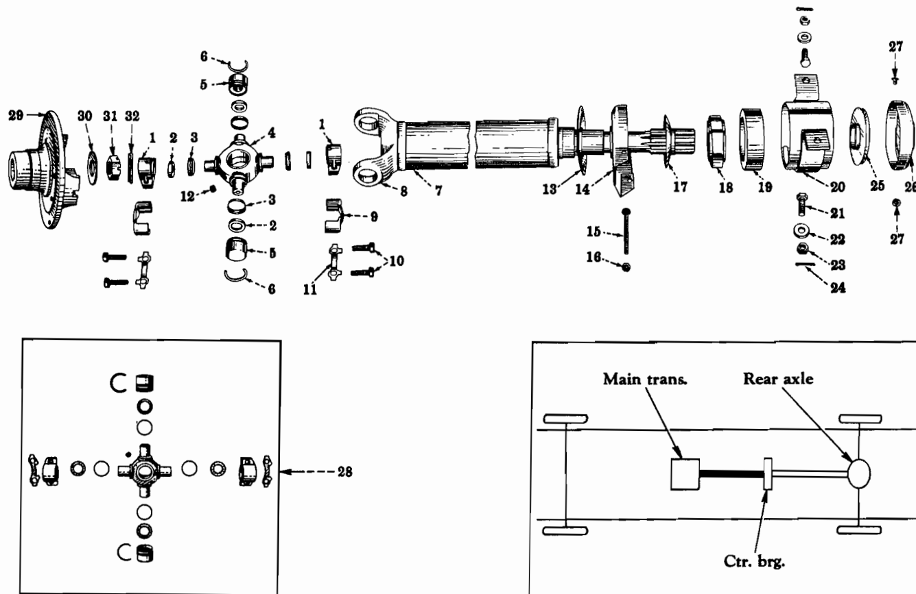
FIG. 06-16 — PROPELLER SHAFT (Mechanics 4-CSR) (Transmission To Center Bearing) (R-130 Series - For 134" W.B., With Transmission Codes 1302, 1303, 1320)
