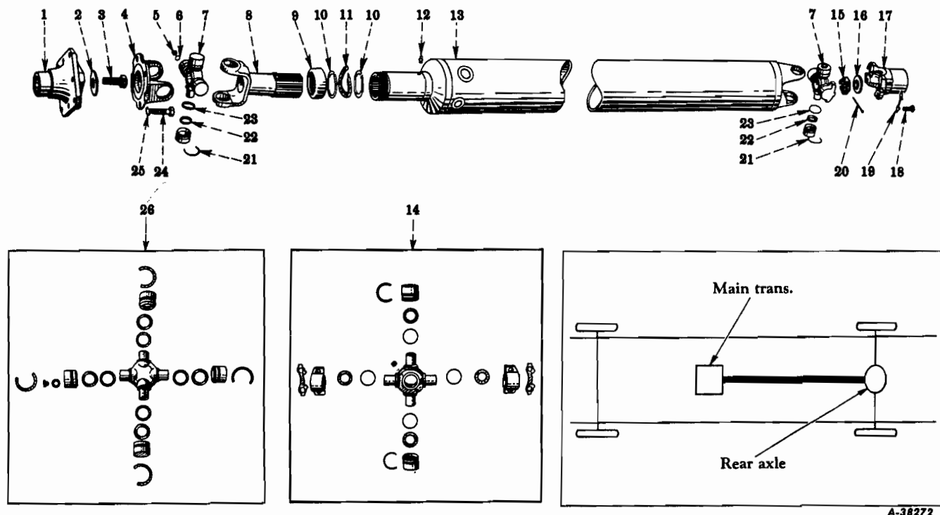
FIG. 06-10 - PROPELLER SHAFT (Mechanics 2-LRCR) (Transmission To Rear Axle) (R-110, R-120 Series - For 127" W.B., With Transmission Code 1374)
