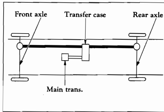
FIG. 06-34 - PROPELLER SHAFT (Spicer 1350, 1400 Series) (Transfer Case To Rear Axle) (R-140-4x4 - Spicer 1350 Series) (R-160-4x4 - Spicer 1400 Series)
