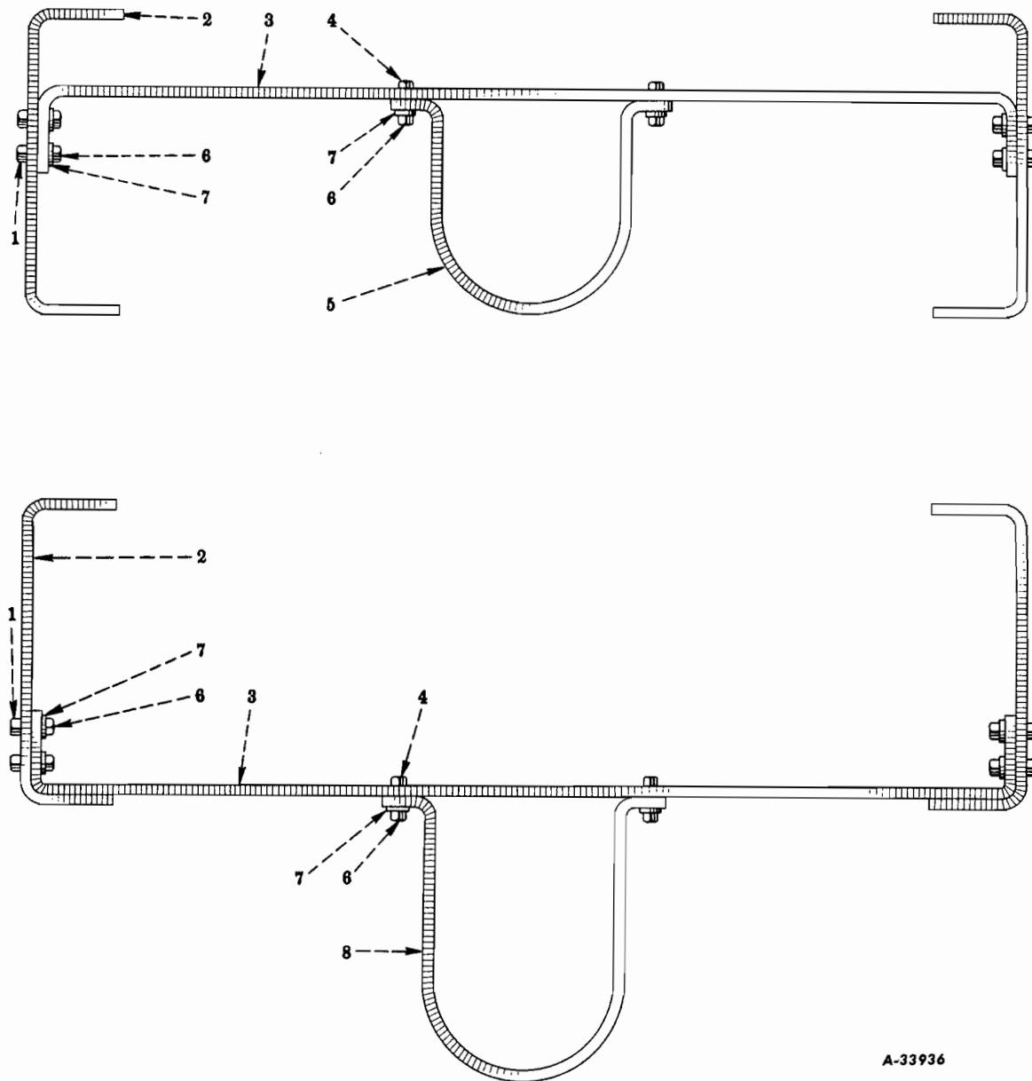
FIG. 06-35 — PROPELLER SHAFT GUARD (Code 0602)
