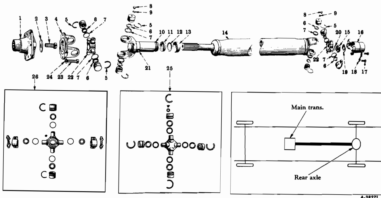
FIG. 06-9 — PROPELLER SHAFT (Mechanics 2-LRCR) (Transmission To Rear Axle) (R-110, R-120 Series - For 115" W.B., With Transmission Code 1374)
