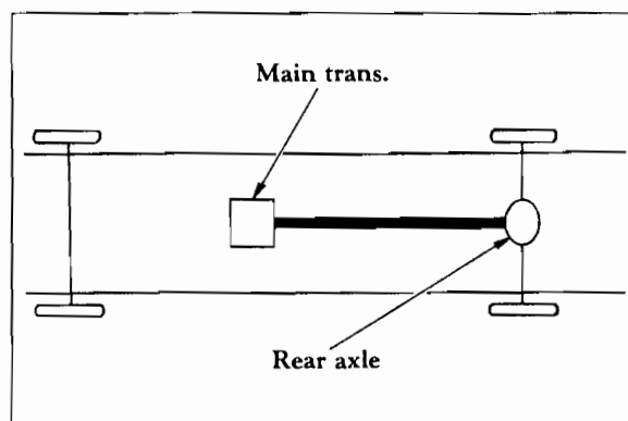
FIG. 06-11 — PROPELLER SHAFT (Mechanics 4-CSR) (Transmission To Rear Axle) (R-130 Series - For 115" W.B., With Transmission Codes 1302, 1303, 1320)
