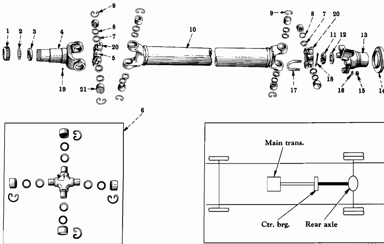
FIG. 06-22 — PROPELLER SHAFT (Spicer 1350 Series) (Center Bearing to Rear Axle) (R-150 Series)
