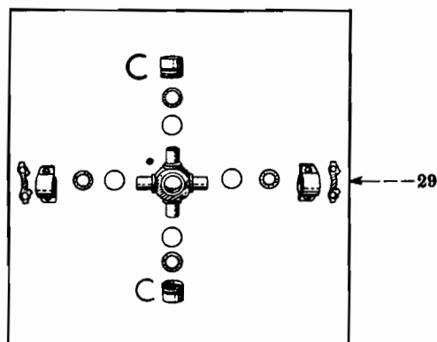
FIG. 06-11 — PROPELLER SHAFT (Mechanics 4-CSR) (Transmission To Rear Axle) (R-130 Series - For 115" W.B., With Transmission Codes 1302, 1303, 1320)
