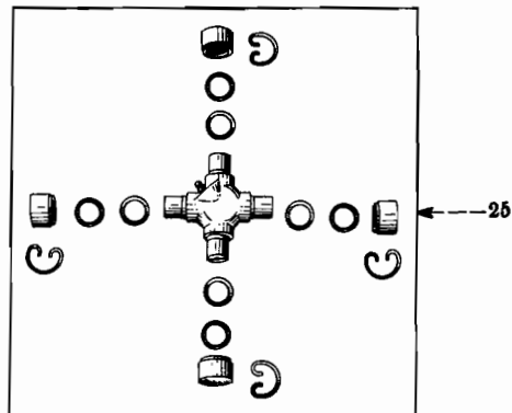
FIG. 06-34 - PROPELLER SHAFT (Spicer 1350, 1400 Series) (Transfer Case To Rear Axle) (R-140-4x4 - Spicer 1350 Series) (R-160-4x4 - Spicer 1400 Series)
