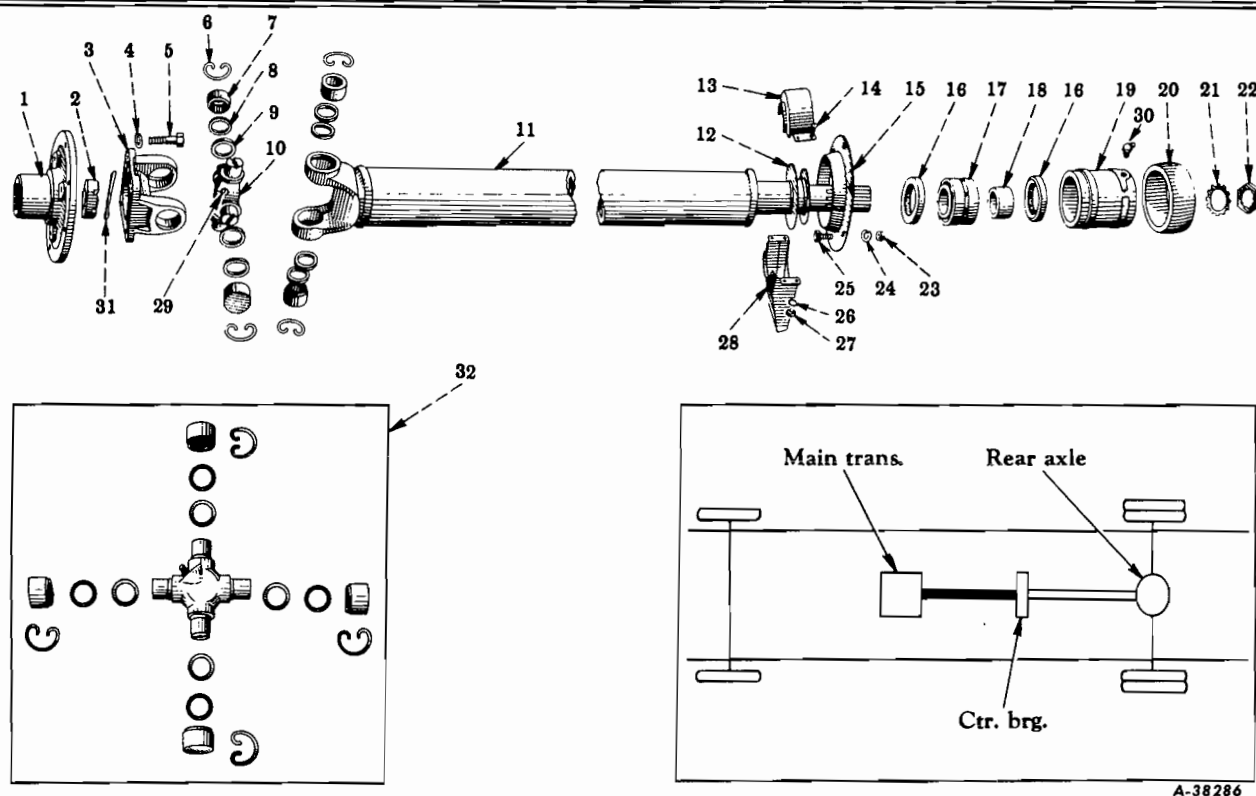
FIG. 06-30 — PROPELLER SHAFT (Spicer 1410, 1350 Series) (Transmission To Center Bearing) (RC-160 Series - With 130, 142, 154, 172" W.B.) (Below 1052 - Spicer 1410 Series) (1052 Up - Spicer 1350 Series)
