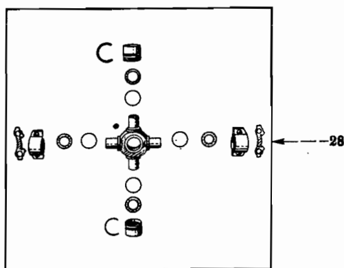
FIG. 06-8 — PROPELLER SHAFT (Mechanics 2-CSR, 2-LCSR) (Transmission To Rear Axle) (R-110, R-120 Series - For 127" W.B., With Transmission Codes 1301, 1302, 1303, 1348)
