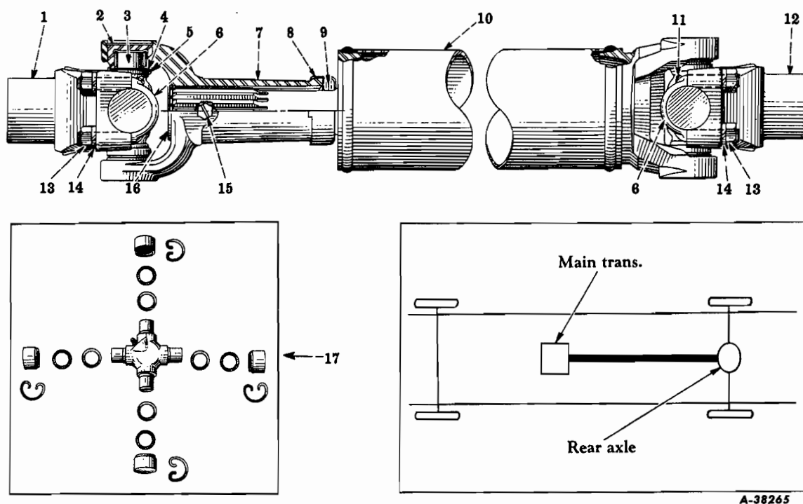
FIG. 06-4 — PROPELLER SHAFT (Spicer 1260 Series) (Transmission To Rear Axle) (R-110 Series - With Transmission Code 1383)
