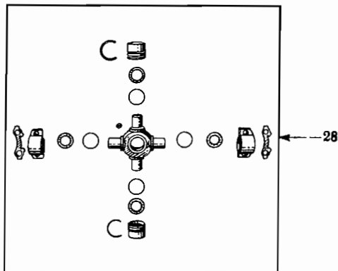
FIG. 06-7 — PROPELLER SHAFT (Mechanics 2-CSR, 2-LCSR) (Transmission To Rear Axle) (R-110, R-120 Series - For 115" W.B., With Transmission Codes 1301, 1302, 1303, 1348)
