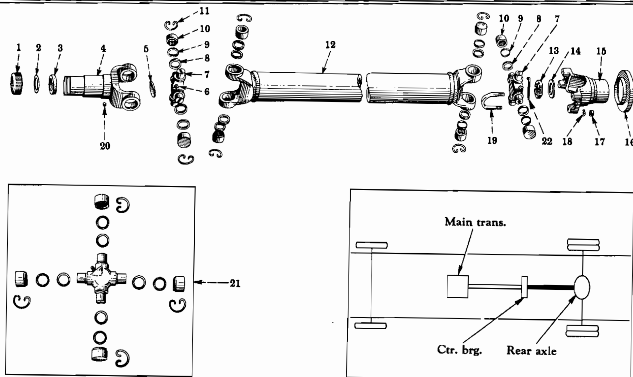
FIG. 06-31 — PROPELLER SHAFT (Spicer 1410, 1350 Series) (Center Bearing To Rear Axle) (RC-160 Series - With 130, 142, 154, 172" W.B.) (Below 1052 - Spicer 1410 Series) (1052 Up - Spicer 1350 Series)
