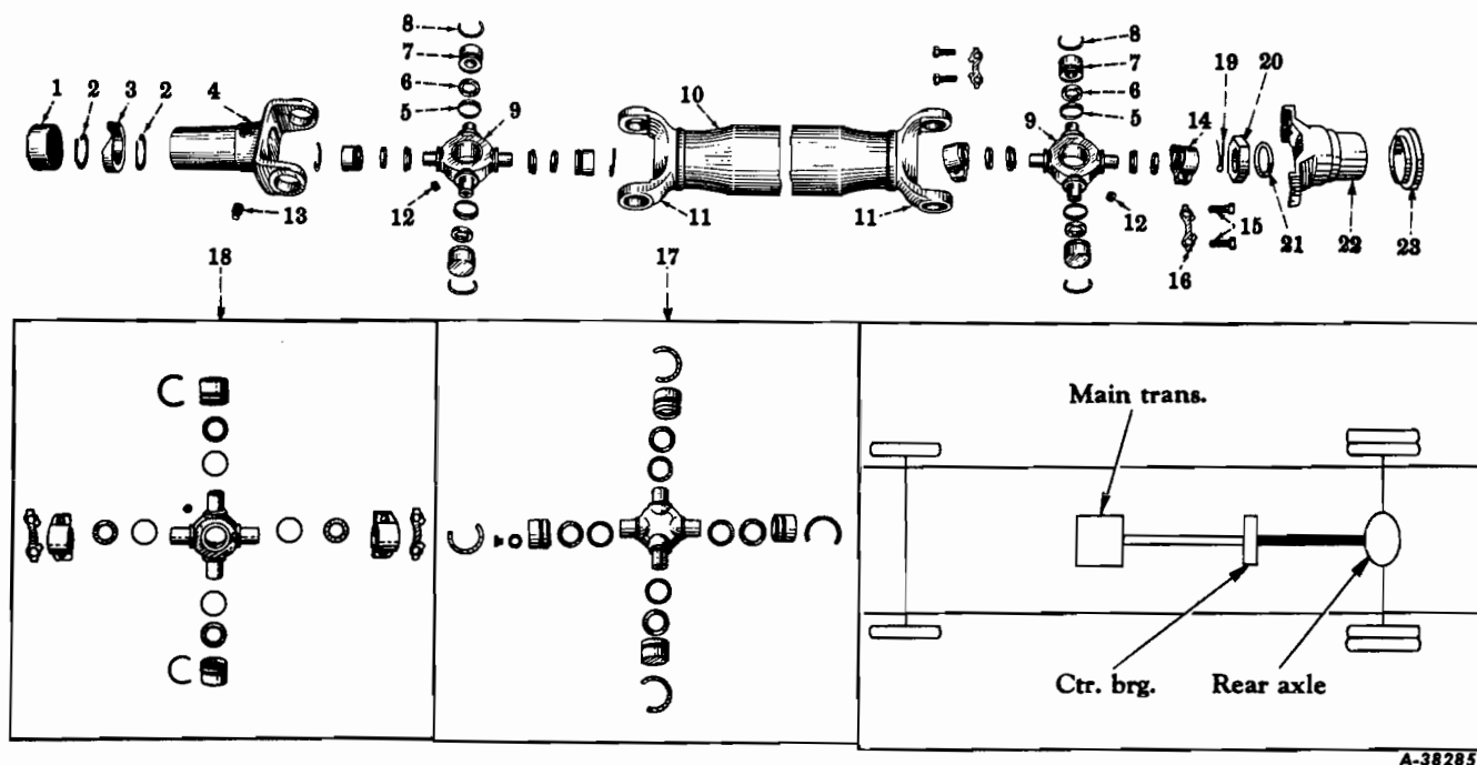
FIG. 06-23 — PROPELLER SHAFT (Mechanics 4-CR) (Center Bearing To Rear Axle) (R-150 Series)
