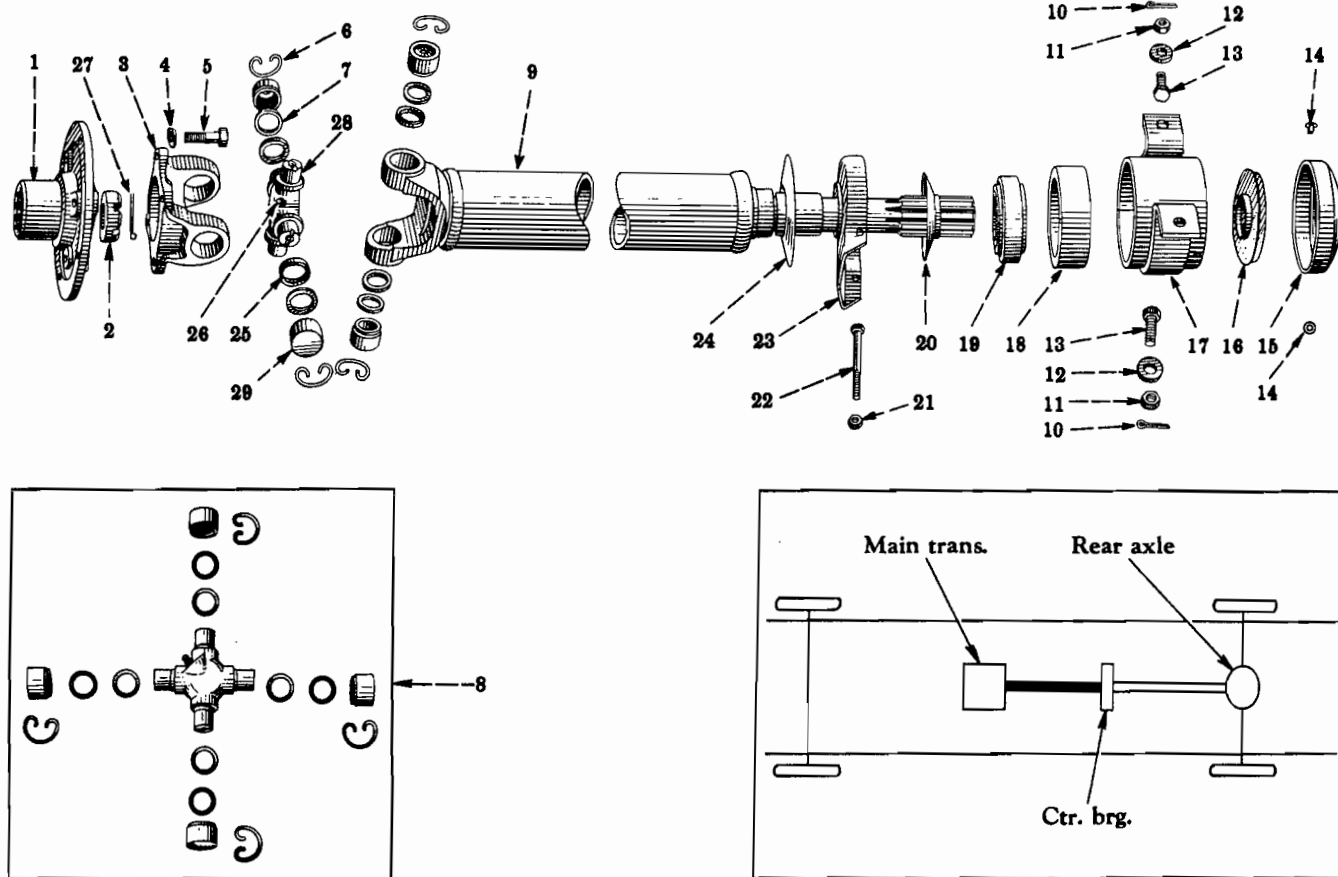
FIG. 06-15 — PROPELLER SHAFT (Spicer 1350 Series) (Transmission To Center Bearing) (R-130 Series - For 134" W.B., With Transmission Codes 1302, 1303, 1320)
