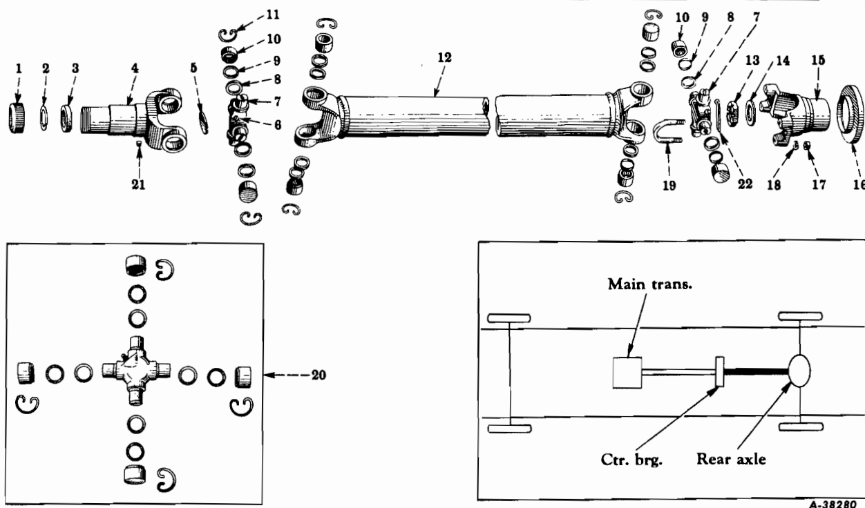
FIG. 06-18 — PROPELLER SHAFT (Spicer 1350 Series) (Center Bearing To Rear Axle) (R-130 Series - For 134" W.B., With Transmission Codes 1302, 1303, 1320)
