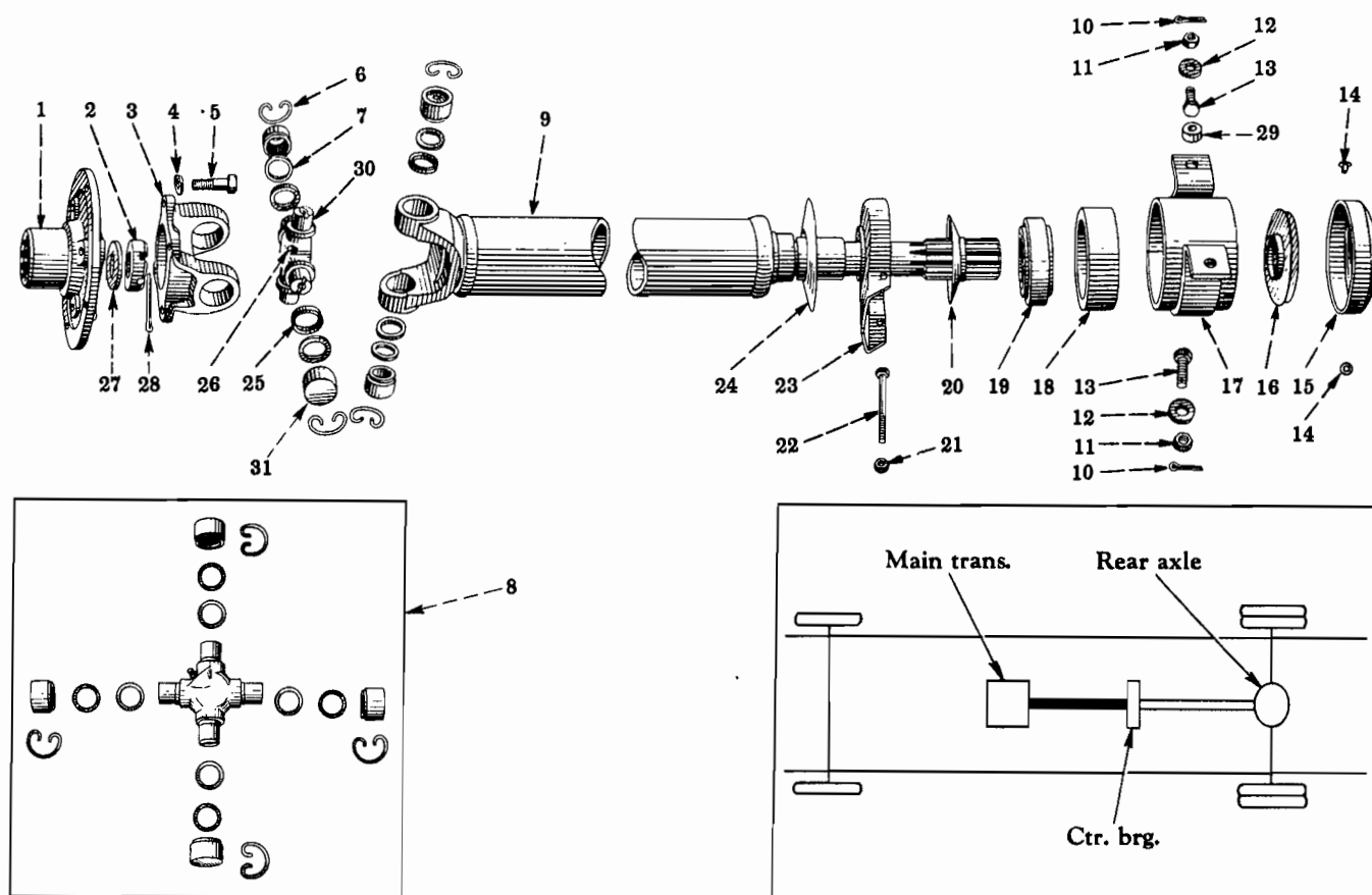
FIG. 06-20 — PROPELLER SHAFT (Spicer 1350 Series) (Transmission To Center Bearing) (R-150 Series)
